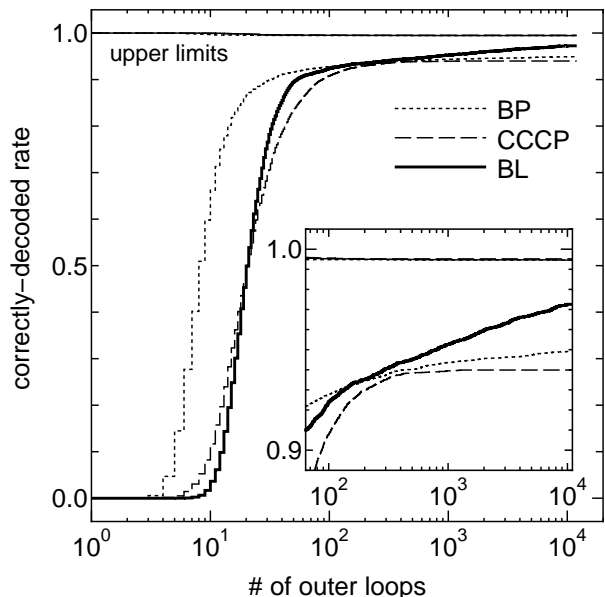
Fig. 3. Time evolution (outer loop steps) of the correctly-decoded rates (lower three lines) and upper limits defined as (1 - [\text{wrongly-decoded rate}]) (upper three lines) for BP, CCCP, and BL algorithms. The data corresponds to the case of E_b/N_0 = 2 in Fig. 2.
