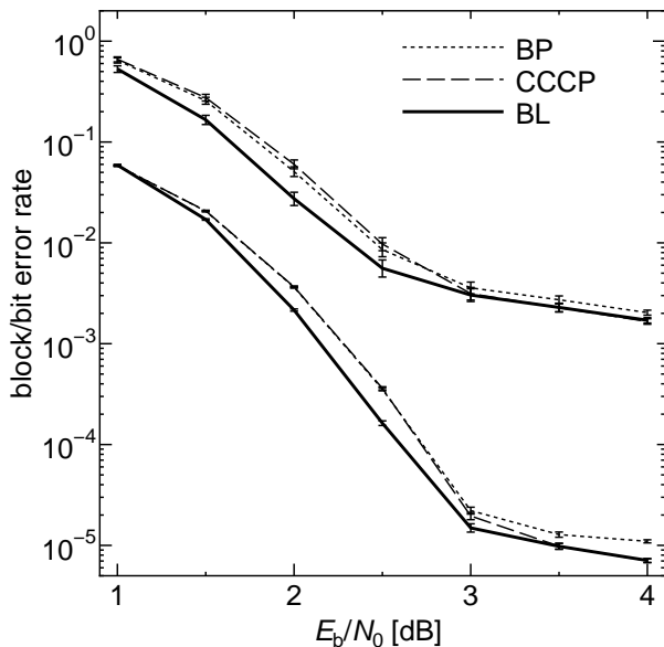
Fig. 2. Block (upper three lines) / bit (lower three lines) error rates of BP, CCCP, and BL algorithms. Configurations were as follows: code length N = 486 , number of parities M = 243 , degree of parity |\mu| = 6 , degree of bit |l| = 3 ((3,6)-regular LDPC), limit of outer loops: 10000 (the limit of loops in the case of BP), number of inner loops fixed as 6 for CCCP and BL, and step width k = 0.3 in BL. E_b/N_0 [dB] is defined as 10 \log_{10}(1/(2\sigma^2(N-M)/N)) . The number of communications were 10^3, 3 \times 10^3, 10^4, 3 \times 10^4, 10^5, 3 \times 10^5 , and 10^6 for E_b/N_0 = 1.0, 1.5, \dots, 4.0 , respectively. Each error bar denotes a 99% confidence interval based on a binomial distribution.
